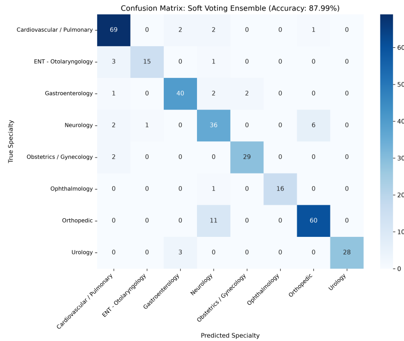
Figure 16: Confusion Matrix of the Soft Voting Ensemble across 8 Clinical Specialties on the Held-Out Test Set
